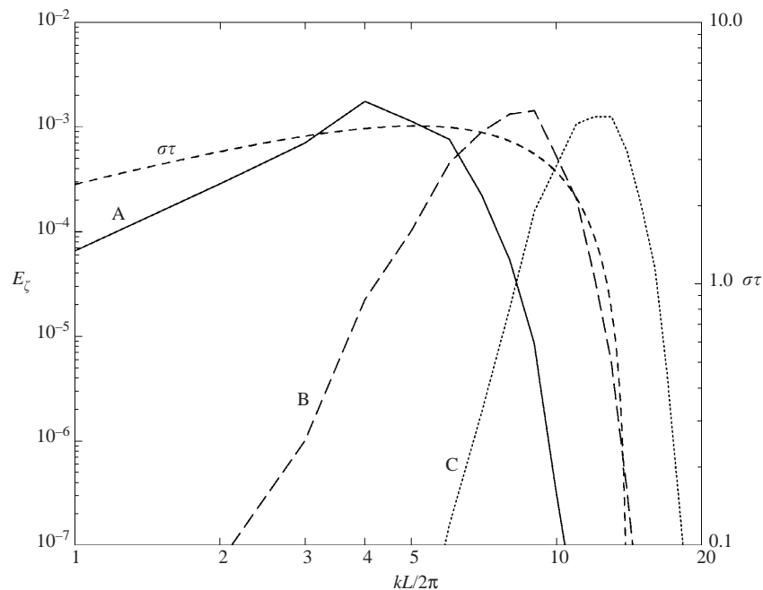
FIGURE 1. Spectra (left axis) of initial interfacial perturbations (18) for Cases A, B, and C. The scaled exponential-growth coefficient (right axis), \sigma(k)\tau , is computed from the linear-stability theory of Duff et al. (1962).
